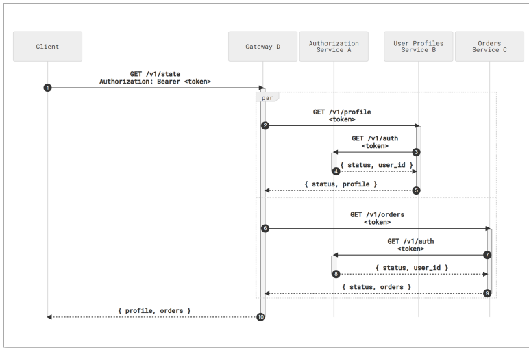
The original microservice mesh
