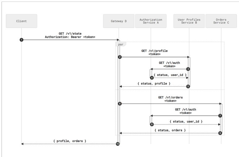
The original microservice mesh
