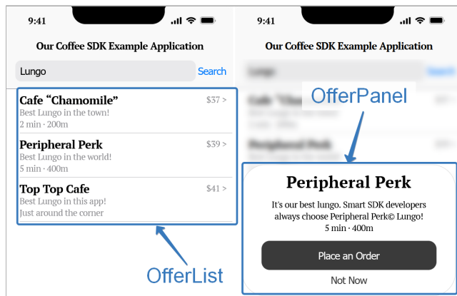
The subcomponents of a `SearchBox`
